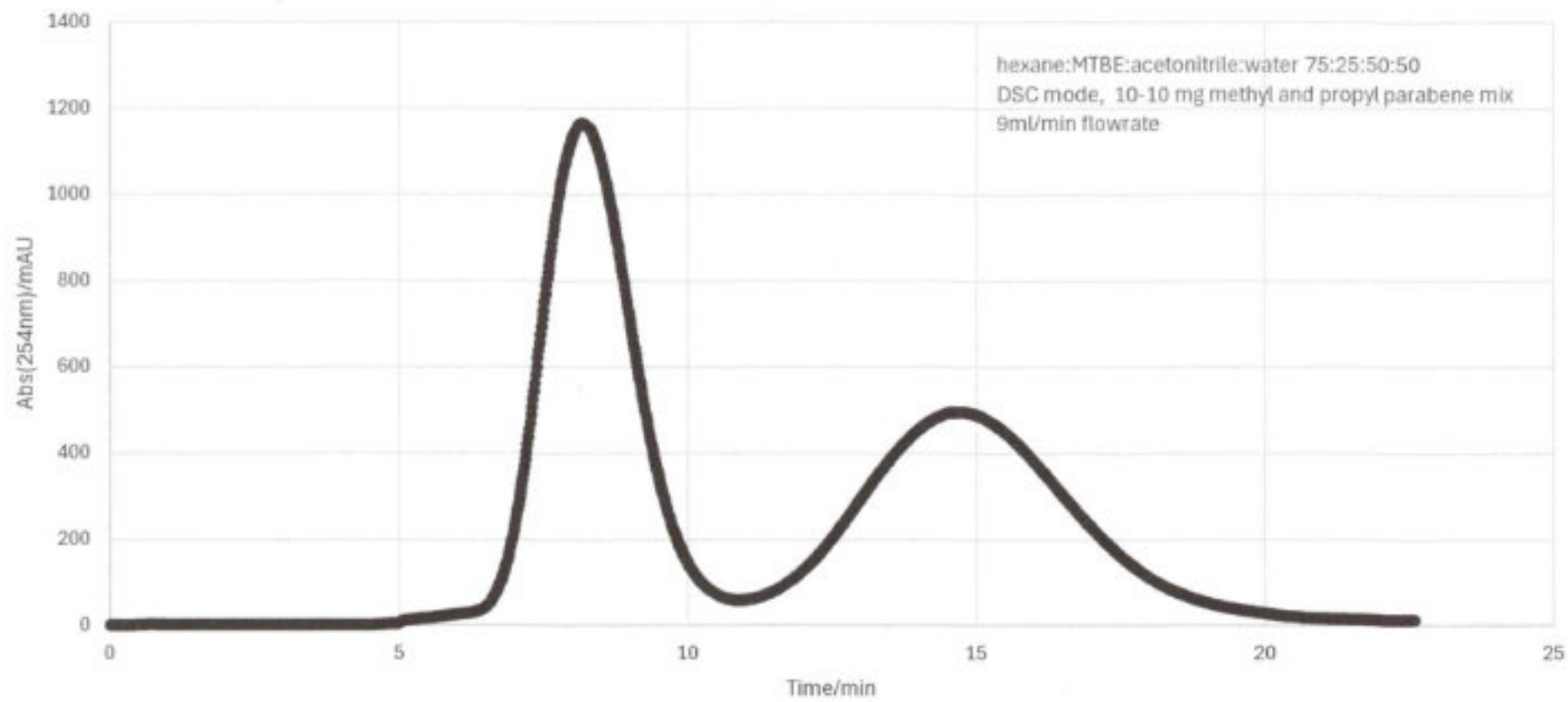
Test chromatogram Midi000038
