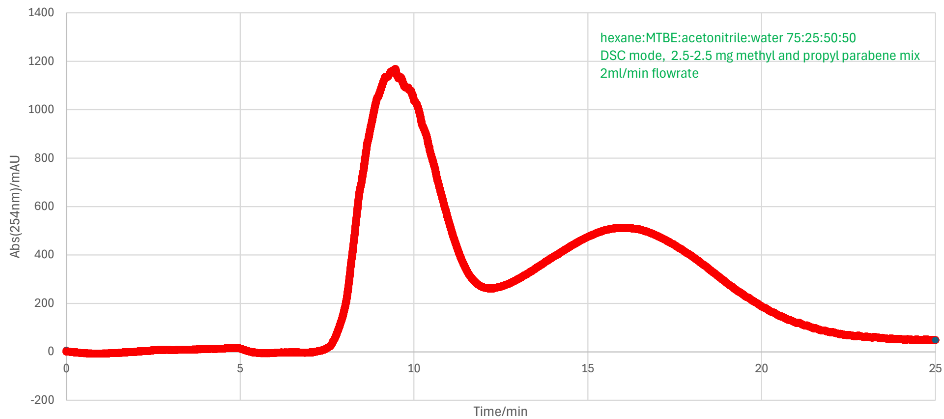
Test chromatogram
